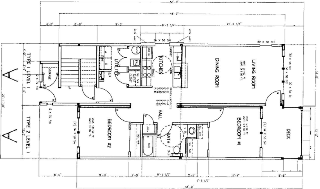
1ST FLOOR 2-BDRM FLAT UNIT
