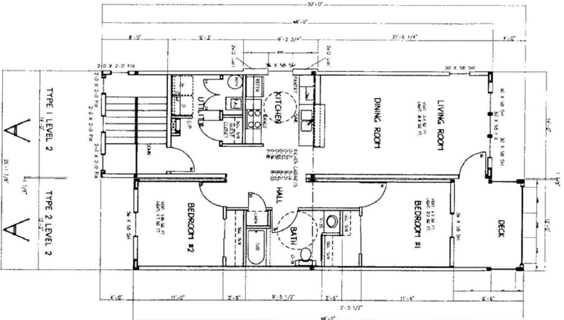
2ND FLOOR 2-BDRM FLAT UNIT
